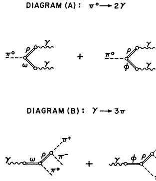
FIG. 1. Diagram (A) shows a model of the neutral pion decay through \rho and \omega(\phi) meson intermediate states and the corresponding diagram for \gamma \rightarrow 3\pi transition amplitude is illustrated in diagram (B). As is easily seen from these diagrams, the ratio of these matrix elements is independent of the vertices corresponding to \omega\rho\pi , \varphi\rho\pi , \omega\gamma , and \varphi\gamma .
