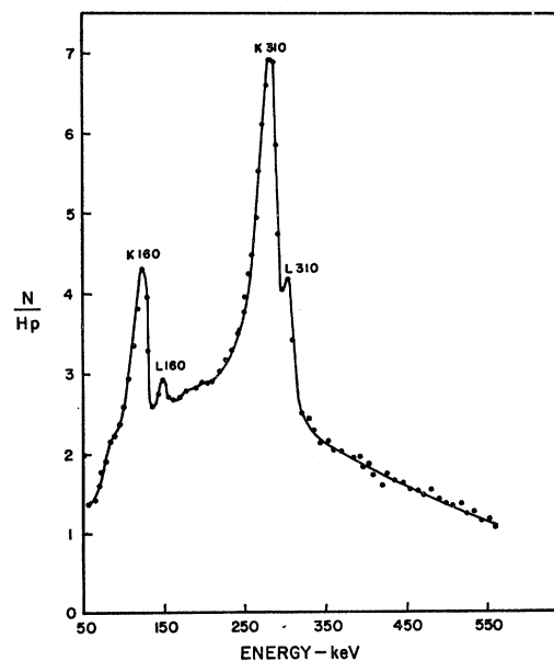
FIG. 1. Internal conversion electron spectrum of \text{Cd}^{117} \rightarrow \text{In}^{117} \rightarrow \text{Sn}^{117} in Siegbahn-Slätis beta-ray spectrometer.
