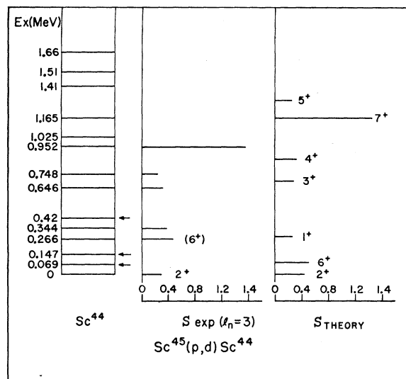
FIG. 6. Energy-level diagram for Sc^{44} and graphical comparison of the experimental results with the theoretical results of McCullen, Bayman, and Zamick for the Sc^{45}(p,d)Sc^{44} reactions. The arrows indicate those levels not observed in the present investigation.
