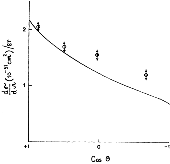
FIG. 1. Differential cross section for \gamma + p \rightarrow K^+ + \Delta^0 . The experimental points are those of Ref. 16.
