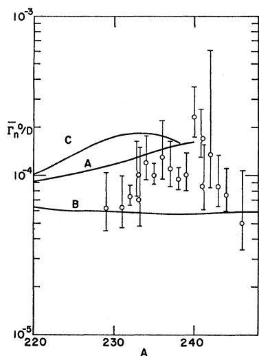
FIG. 3. The strength function \bar{\Gamma}_n^0/D for the nuclides with nucleon numbers A between 220 and 248. The curves are all from Chase, Willets, and Edmonds (Ref. 9). Curve A is based on a spheroidal potential that provides the best fit to the data near A = 160 . Curve B is based on a spherical potential. Curve C corresponds to the same set of parameters as curve A except for the quadrupole deformation which is 33% larger for C. The values of \bar{\Gamma}_n^0/D are from the results of the many workers listed in Table III.
