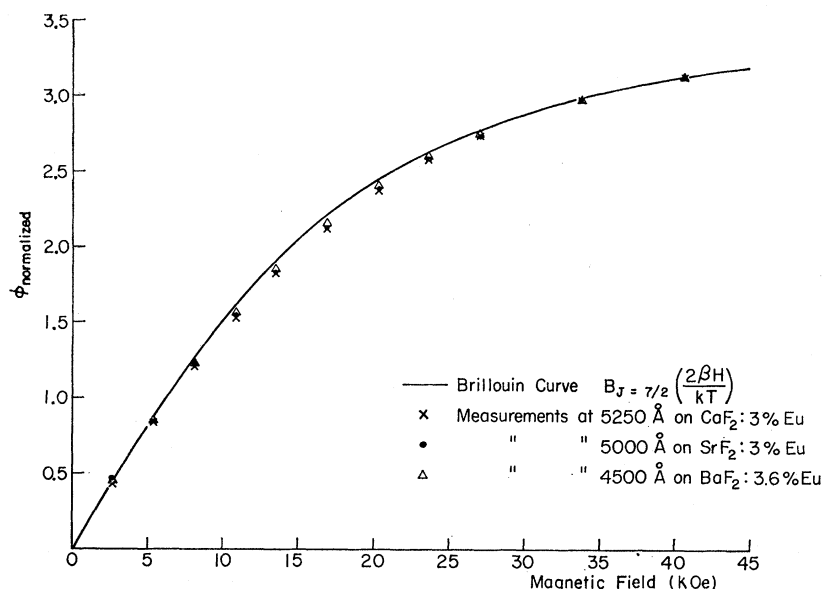
FIG. 1. Measurements of rotation versus magnetic field on \text{CaF}_2 : 3% Eu, \text{SrF}_2 : 3% Eu, and \text{BaF}_2 : 3.6% Eu at 4.2°K. The rotations are normalized by matching to the Brillouin curve at 40.66 kOe. They shift slightly towards the Brillouin curve as the frequency moves towards the absorption band. The samples, 2.5 mm in length, were grown in a hydrogen atmosphere.
