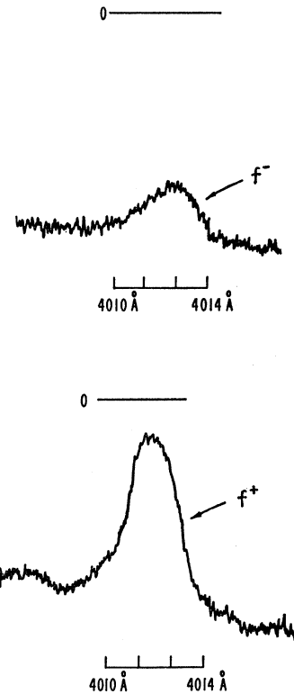
FIG. 6. Circular dichroism of the 4011.5 \text{ \AA} line of \text{Eu}^{2+} in \text{SrF}_2:0.007\% \text{Eu} at 4.2^\circ\text{K} and 21.6 \text{ kOe} .
