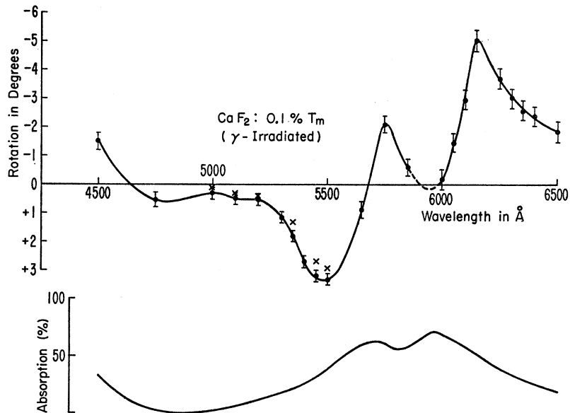
FIG. 7. Rotatory dispersion of \text{CaF}_2:0.1\% \text{Tm} at 4.2^\circ\text{K} and 21.6 \text{ kOe} . The sample, 2.5 \text{ mm} in length, were \gamma radiated. \square Measurements made 3 days after \gamma irradiation. \times Measurements made 24 days after \gamma irradiation.
