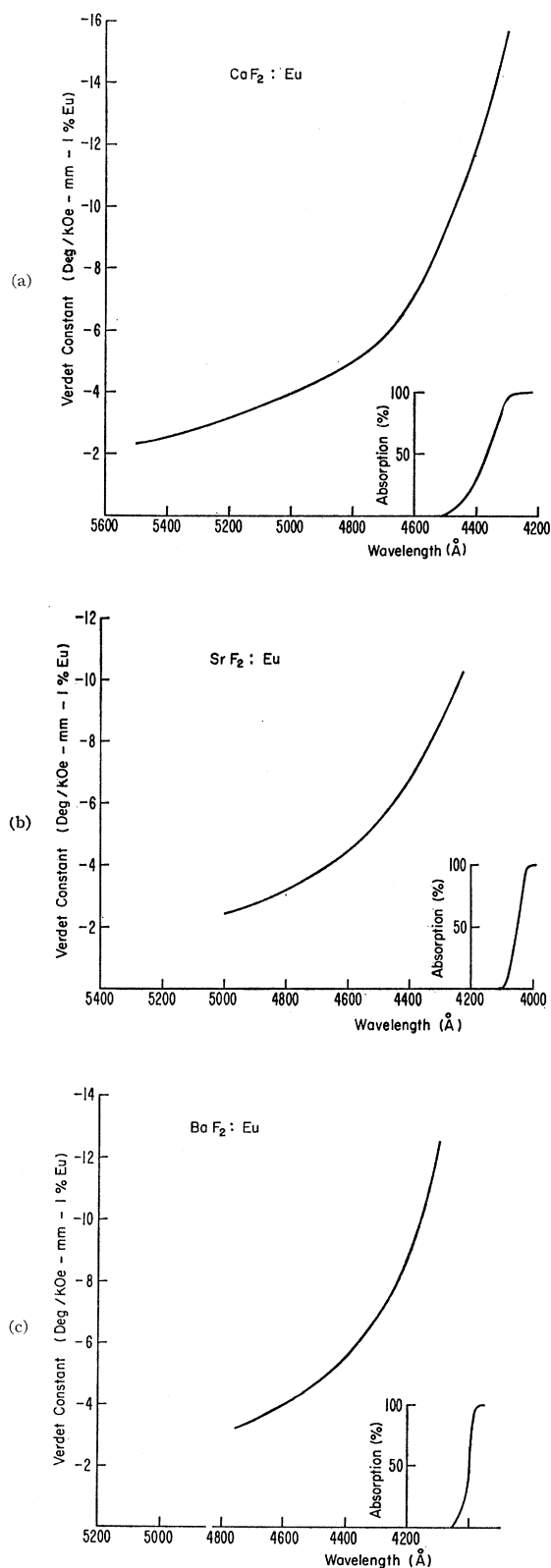
FIG. 2. Rotatory dispersion curves at 4.2°K and 2.71 kOe on (a) \text{CaF}_2 : 3% Eu; (b) \text{SrF}_2 : 3% Eu; (c) \text{BaF}_2 : 3.6% Eu.
