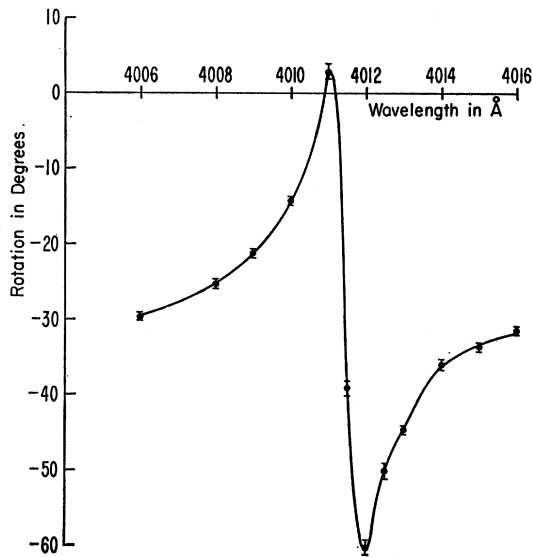
FIG. 5. Rotatory dispersion of \text{SrF}_2:0.007\% \text{Eu} about the 4011.5 \text{ \AA} line of \text{Eu}^{2+} at 4.2^\circ\text{K} and 21.6 \text{ kOe} .
