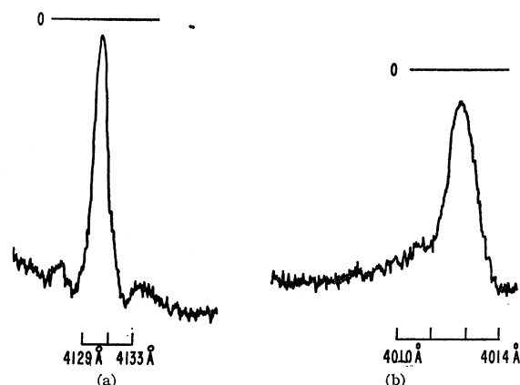
FIG. 3. Narrow spectral lines of \text{Eu}^{2+} in \text{CaF}_2 and \text{SrF}_2 at 4.2°K. The samples, 2.5 mm in length, were grown in a hydrogen atmosphere. (a) \text{CaF}_2 : 0.005% Eu; (b) \text{SrF}_2 : 0.007% Eu.
