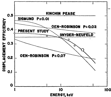
FIG. 1. Displacement efficiency reduction due to channeling.
