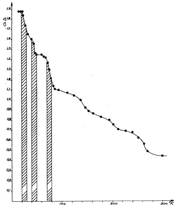
FIG. 4. Annealing behavior of F band in a crystal kept for 12 h at 650^{\circ}\text{C} in a He atmosphere before irradiation. Irradiation at 45 kV and 30 mA for 21 h, 0.5-mm Al filter. Sample thickness 0.82 mm.
