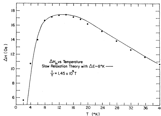
FIG. 5. Comparison of slow relaxation theory for ferromagnetic-resonance linewidth with experiment at low temperatures. The solid curve is a plot of Eq. (1) for \Delta E/k = 8^\circ\text{K} and 1/\tau = 1.45 \times 10^9 T .
