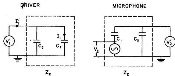
FIG. 3. Four terminal reciprocity network. C_t : capacitance of a transducer. C_g : cable capacitance. C_t and C_g were identical to within \frac{1}{2}\% for both transducers. Z_d : combined impedance of a transducer and its cable. V_2' : generated microphone voltage. V_2' : measured microphone voltage. I_1 : actual driving current. I_1' : measured driving current. V_1' : measured driving voltage.
