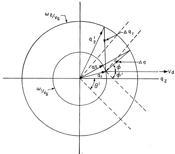
FIG. 7. Higher order electron phonon processes. These processes can be described in terms of the emission or absorption of apparent phonons. Two such processes are shown which have different changes in wave vector q_2 - q_1 or q_2' - q_1 for a fixed energy difference \omega_2 - \omega_1 . This is equivalent to a variable apparent velocity. The cone \varphi' is the gain cone for these apparent phonons. Emission or absorption of these apparent phonons will be more probable depending on whether q_2 is inside or outside \varphi' . \theta' is the gain cone for first-order processes.
