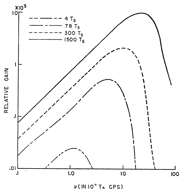
Fig. 5. Relative stimulated momentum gain as a function of phonon frequency. The function r_2(\nu) is plotted for T=4T_s , 78T_s , 300T_s , and 1500T_s . These temperatures correspond roughly to liquid helium, liquid nitrogen, and room temperature for m^* \approx m_0 , and room temperature for m^* \approx 0.2m_0 .
