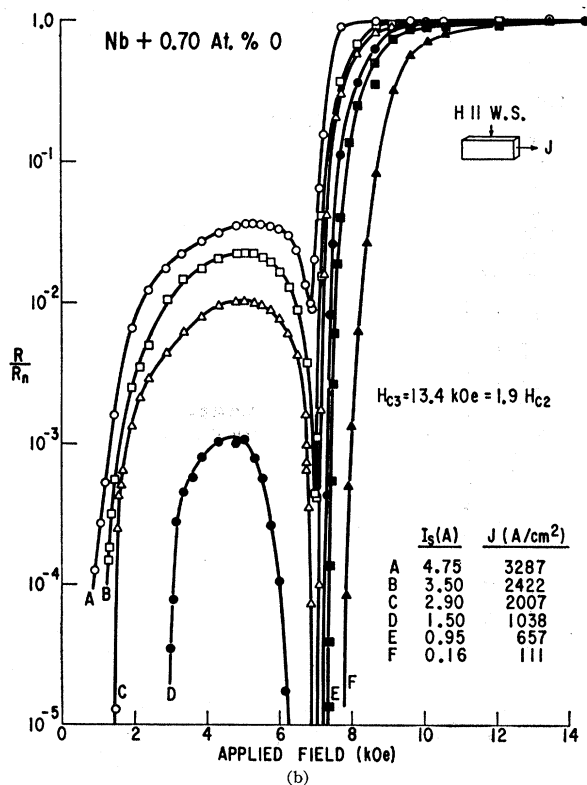
FIG. 8. The resistance characteristics R/R_n as a function of applied transverse field at 4.2°K for a cold-worked ribbon (0.032×0.007 in.) containing 0.70 at.% oxygen (a) with field perpendicular to wide side; (b) with field parallel to the wide side. H_{c3} values were evaluated at J=111 A/cm 2 .
