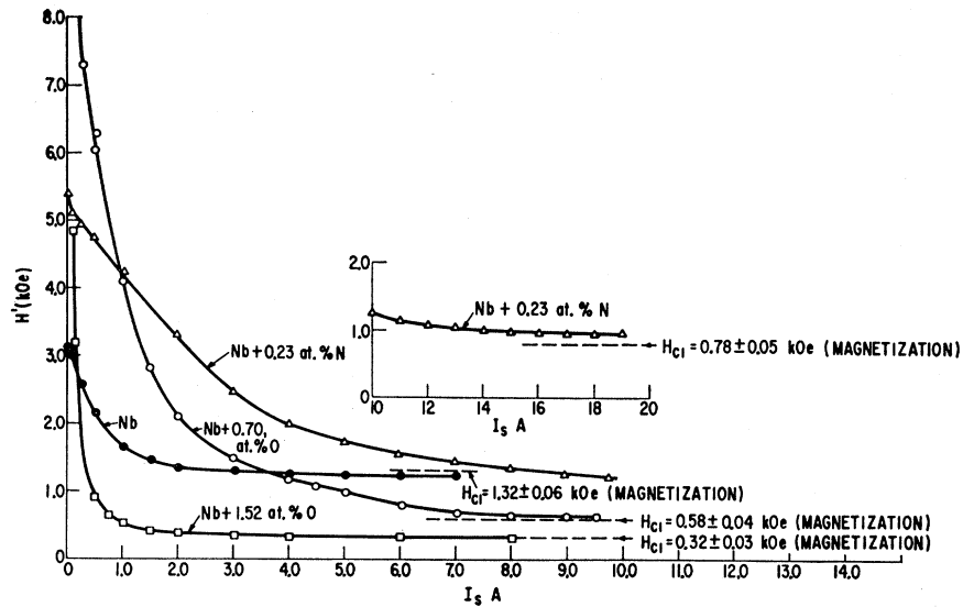
FIG. 5. The transverse field H' required for the initial appearance of resistance ( R/R_n \lesssim 1 \times 10^{-3} ) at 4.2°K as a function of specimen current I_s (amperes). The values of H_{c1} are evaluated from the magnetization curve.
