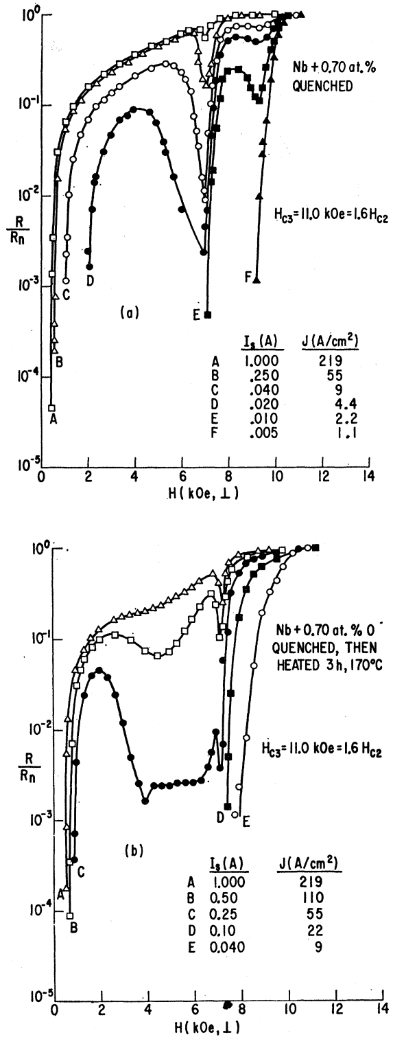
FIG. 20. The resistance characteristics R/R_n of niobium wire (0.030-in. diam) containing 0.70 at.% oxygen ( T=4.2^\circ\text{K} ); (a) quenched in helium exchange gas from an homogenization temperature of approximately 1200^\circ\text{C} ; (b) then heated 3 h at 170^\circ\text{C} . H_{c3} evaluated at J=10 \text{ A/cm}^2 .
