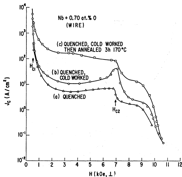
FIG. 17. Threshold current-density field behavior of the same specimens shown in Fig. 16 ( T=4.2^\circ\text{K} ).
