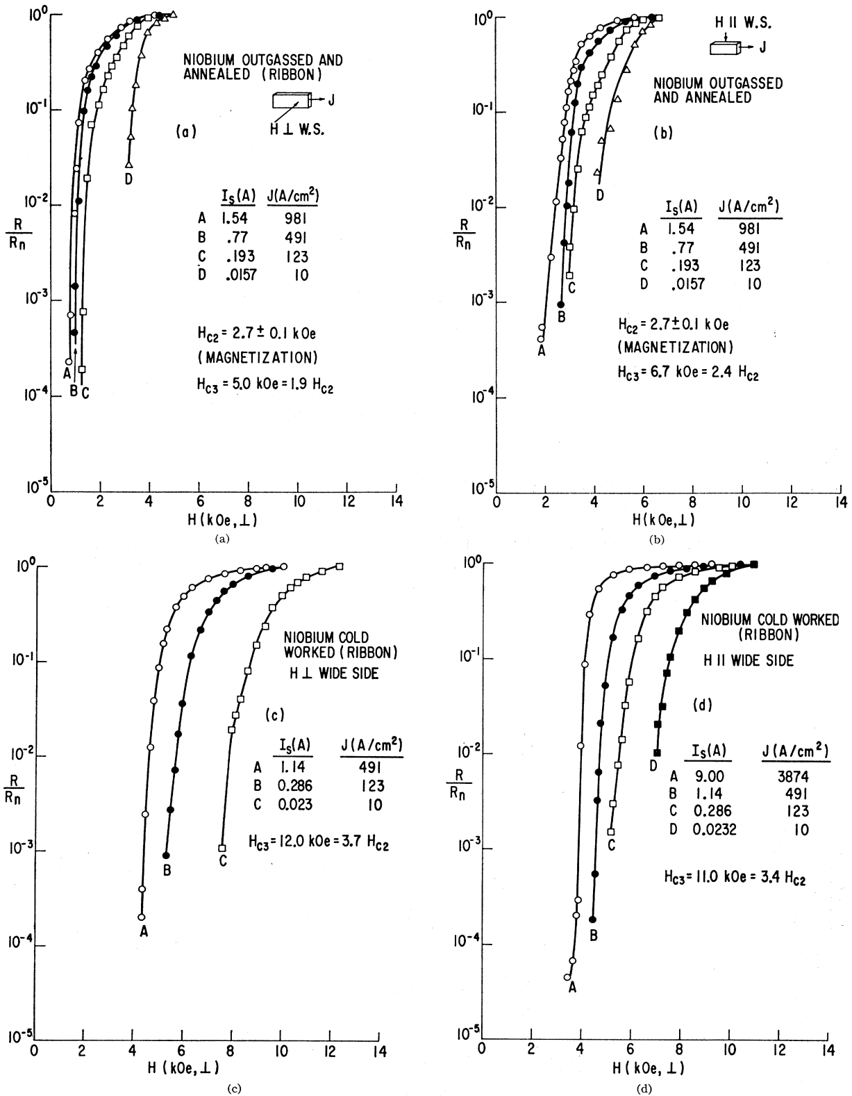
FIG. 11. The resistive characteristics R/R_n , as a function of applied transverse field at 4.2°K for niobium ribbons (0.032×0.007 in.) containing less than 5 ppm interstitials: (i) annealed; (a) field perpendicular to wide side (b) parallel to wide side; (ii) cold worked by uniformly compressing a 0.030-in. diam wire (ribbon dimensions 0.032×0.007 in.); (c) field perpendicular to wide side; and (d) field parallel to wide side. H_{c3} values are evaluated at J \cong 10 A/cm 2 .
