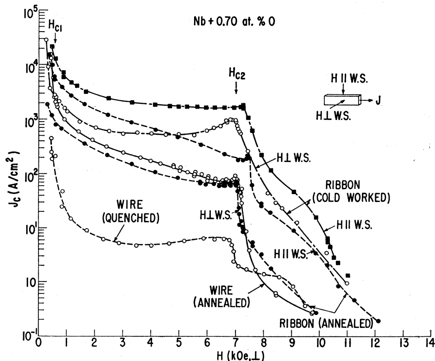
FIG. 14. Threshold current-density field behavior of several specimens of niobium wire (0.030-in. diam) and ribbons (0.032×0.007 in.) containing 0.70 at.% oxygen at 4.2°K. H_{c1} and H_{c2} determined from magnetization data.
