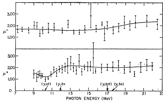
FIG. 6. Energy dependence of the quantities \mu^+ and \mu^- . The error bars represent the standard deviation computed from the propagation of the statistical error in P_N through Eq. (10).
