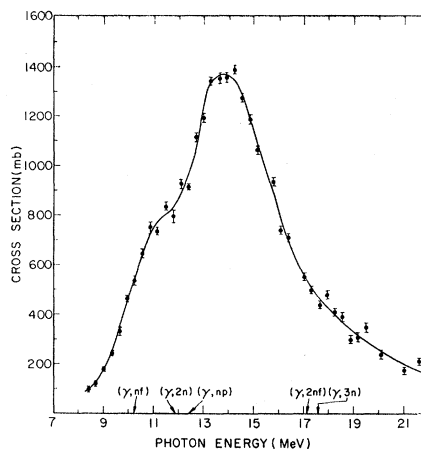
FIG. 5. Total neutron-emission cross section σ(γ,N) for U 235 . These data were obtained by taking the difference between the neutron-yield curves of Fig. 4. The statistical errors on the points represent the standard deviation of the measurements with positrons. The thresholds for various reactions which emit neutrons are also shown.
