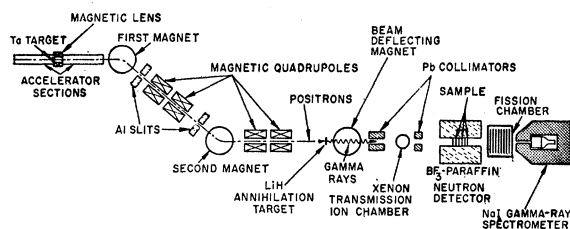
FIG. 1. Experimental apparatus for the photodisintegration measurements (not to scale). For the photofission measurements, the fission chamber was placed between the neutron detector and the gamma-ray spectrometer. The spark chamber was at the same position with the calibrated ionization chamber immediately behind the neutron detector. Neutron- and gamma-ray shielding has been omitted.
