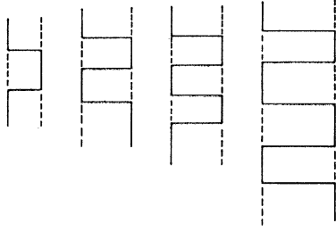
FIG. 2. Higher-order ladder diagrams which generate the nucleon Regge pole.
