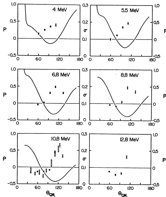
FIG. 1. Polarization and cross section of protons elastically scattered by \text{He}^3 . The present polarization data are represented by dots. The open rectangles are the measurements of Rosen and Brolley at 10 MeV (Ref. 13). The solid lines are smooth curves drawn through the present cross-section measurements (Table II). The cross-section scale is in the center-of-mass system and is given in units of barns per steradian.
