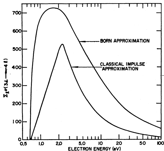
FIG. 4. Total cross sections for excitation of the n=4 ( l=0, 1, 2 , or 3 ) state of hydrogen obtained from the Born approximation 16 and the classical impulse approximation.
