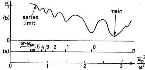
FIG. 4. (a) Position of resonances assuming a density distribution of Fig. 2 and \omega_{pm}^2 = 1.5\langle\omega_p\rangle_{av}^2 . (b) A schematic curve obtained from Dattner's experiment; microwave frequency 1.5 GHz, mercury temp. 20°C, tube diameter 32.4 mm. P_T denotes the transmitted power.
