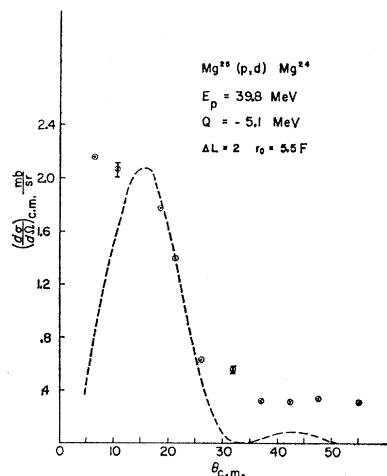
FIG. 11. Angular distribution of deuterons from Mg^{25}(p,d)Mg^{24} , ground state.
