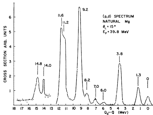
FIG. 3. Energy spectrum of deuterons from (p,d) reactions on natural magnesium.
