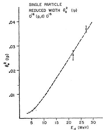
FIG. 9. Dependence of the single-particle reduced width \theta_0^2(1p) on deuteron bombarding energy as measured from O^{16}(p,d)O^{15} . Open circles are data of Ref. 10.
