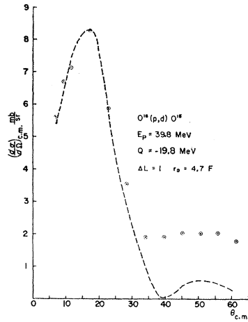
FIG. 8. Angular distribution of deuterons from O^{16}(p,d)O^{15*} , 6.4-MeV state.
