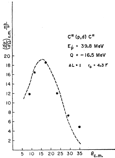
FIG. 6. Angular distribution of deuterons from C^{12}(p,d)C^{11} , ground state.
