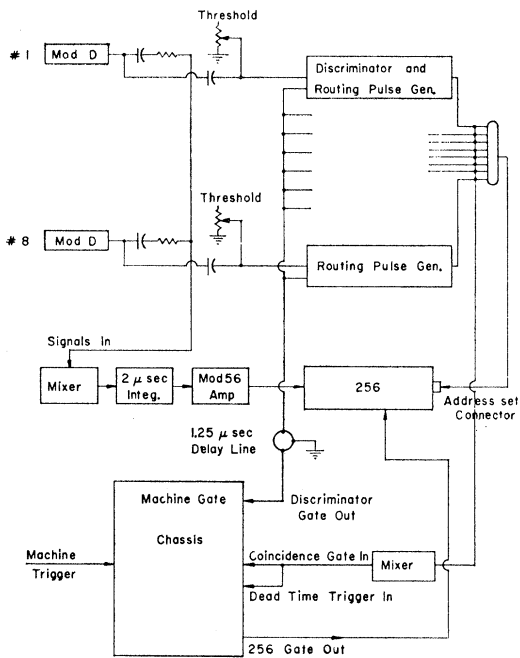
FIG. 1. Pulse-analyzing circuit.
