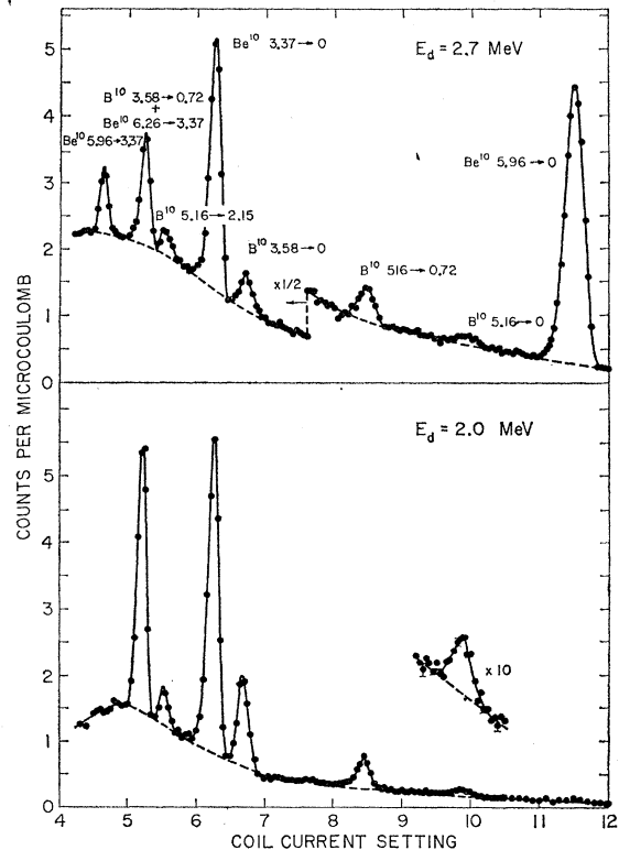
FIG. 3. Magnetic lens pair spectrometer results for Be^9 + d at E_d = 2.7 MeV (upper curve) and 2.0 MeV (lower curve). The pair lines are identified by the nucleus and the energy levels (in MeV) to which they are assigned. The resolution (full width at half-maximum) for these spectra is 2.95%.
