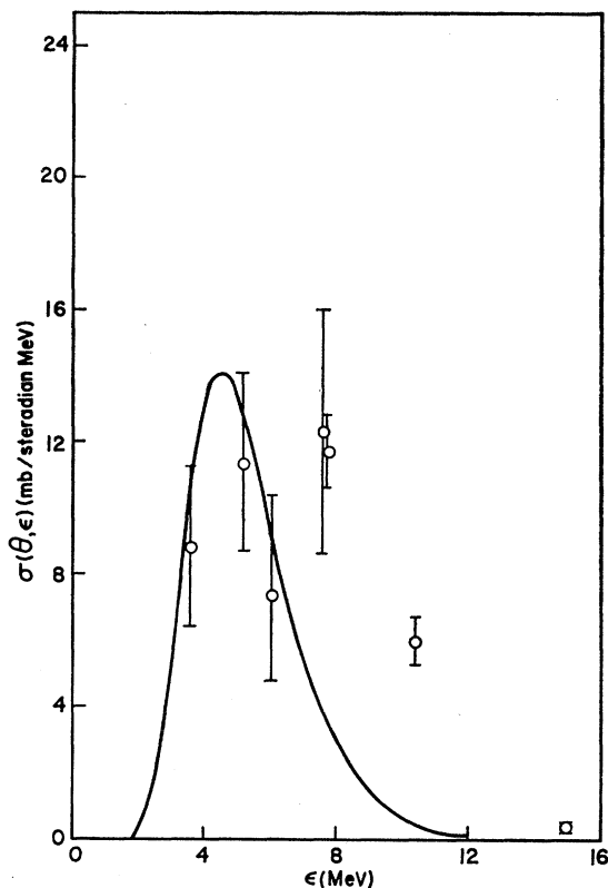
FIG. 4. Proton cross sections at 0^\circ . (The curve represents compound nucleus contribution based on the nuclear temperature of 1.0 MeV).
