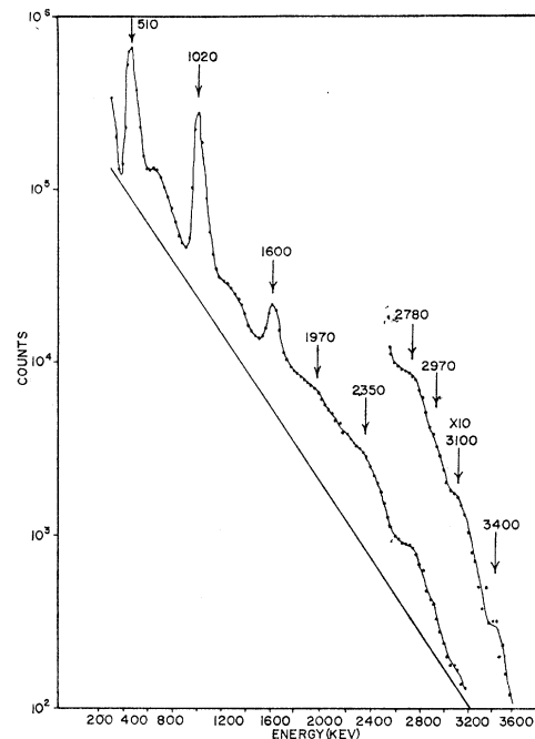
FIG. 4. The gamma-ray spectrum of a mixed source of \text{Xe}^{122} — \text{I}^{122} , \text{Xe}^{125} and \text{Xe}^{127} with the source inside the well of a 3 in. \times 3 in. NaI (Tl) crystal. The solid line is the estimated intensity of the bremsstrahlung due to positron annihilation.
