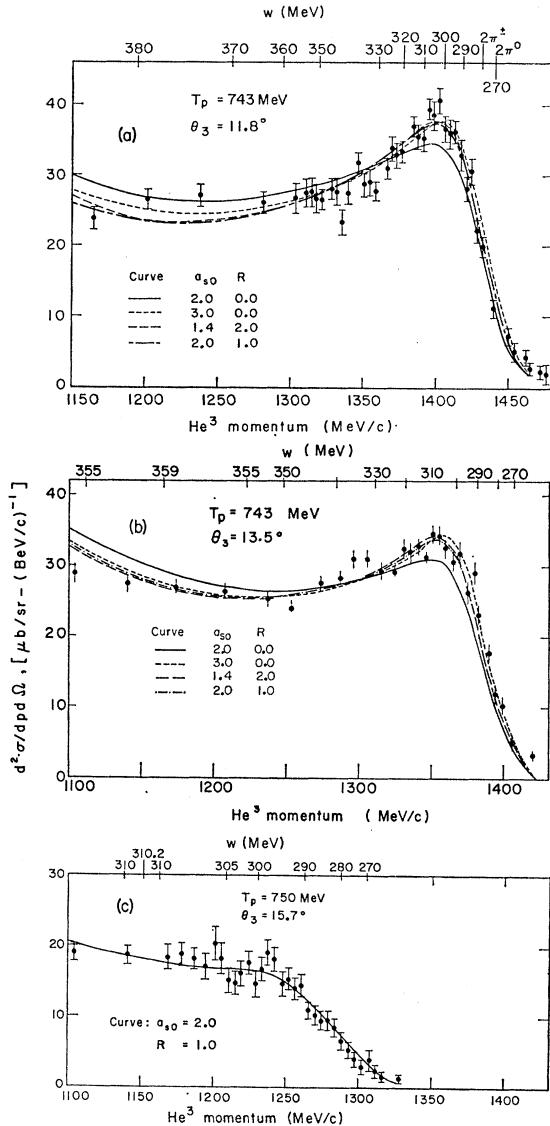
FIG. 14. Fits to the experimental data showing the effect of varying the symmetrization radius R and the scattering length a_{s0} . All fits shown are more or less acceptable except the case a_{s0} = 2.0 , R = 0.0 .
