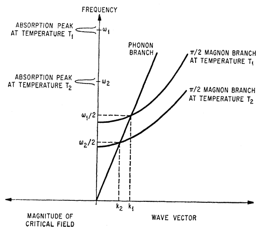
FIG. 2. Plot showing the crossing of the phonon spectrum with the \frac{1}{2}\pi magnon branch at temperatures T_1 and T_2 . Also indicated are the frequencies at which the peaks in the critical field occur.
