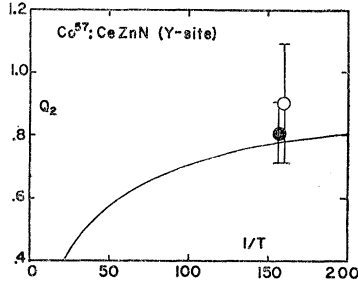
FIG. 5. Attenuation coefficient Q_2 due to intermediate state reorientation following decay of \text{Co}^{57} in Y sites of Ce-Zn nitrate at 1/T^* = 157 , compared with a curve computed from Steenberg's theory of reorientation by static, isotropic hfs coupling in the hard-core limit. The open circle is Q_2 from the 137-keV data; the closed circle represents Q_2 from 123-keV results.
