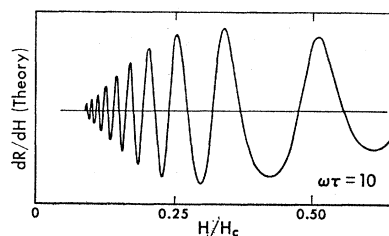
FIG. 1. Absorption derivative curve for a specimen having an isotropic cyclotron effective mass and \omega_{rf}\tau = 10 , according to the theory of Azbel' and Kaner.
