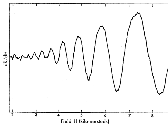
Fig. 2. Experimental absorption derivative trace obtained from a lightly etched single crystal of potassium. Essentially identical traces were obtained for all directions of \mathbf{H} in the (110) plane. This curve closely resembles the theoretical curve in Fig. 1.
