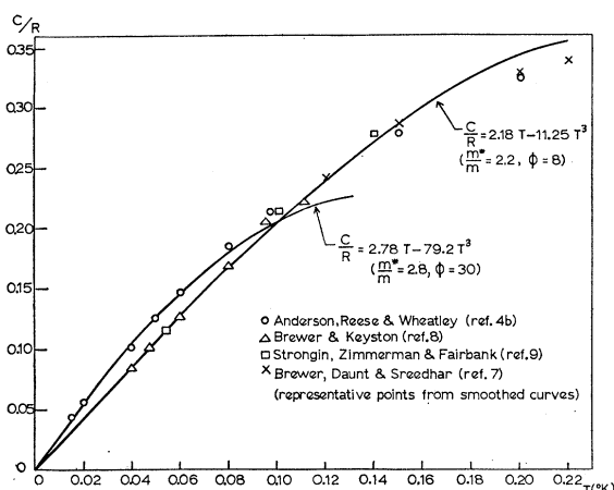
FIG. 2. Specific heat C of liquid \text{He}^3 divided by gas constant R near zero pressure. Experimental values for the parameter \phi appearing in Eq. (24) are determined by fitting curves of the form C/R = cT - dT^3 to the lowest temperature data, with T in ^\circ\text{K} . From (24), c = (\pi^2/2)(m^*/5m) and d = (3\pi^4/20)(m^*/5m)^3(1+\phi) since T_{F0} , the degeneracy temperature for an ideal Fermi gas with the same mass and density as liquid \text{He}^3 at zero pressure, is approximately 5.0^\circ\text{K} .
