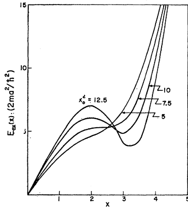
FIG. 1. Excitation energy for various values of x_0^2 .
