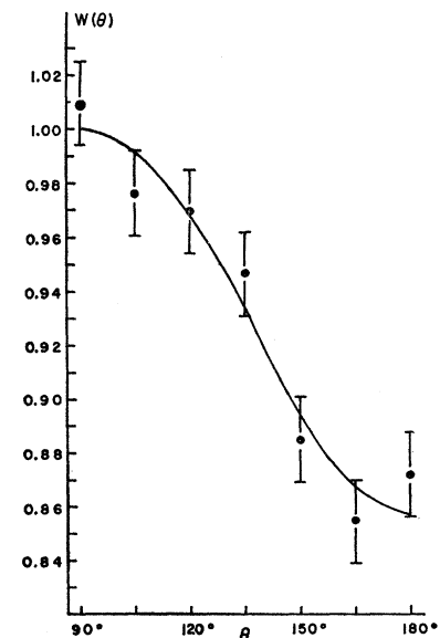
FIG. 7. 329-1597-keV skip correlation of \text{Ce}^{140} .
