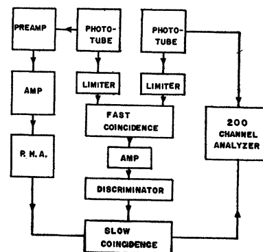
Fig. 1. Block diagram of the apparatus.
