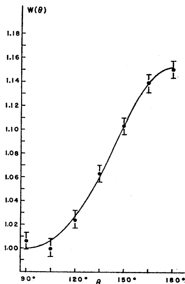
FIG. 4. Directional correlation of the 487-1597-keV cascade of Ce 140 .
