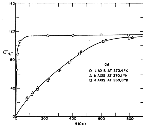
FIG. 3. Magnetic moment per gram versus internal magnetic field for the a -, b -, c -axis crystals.
