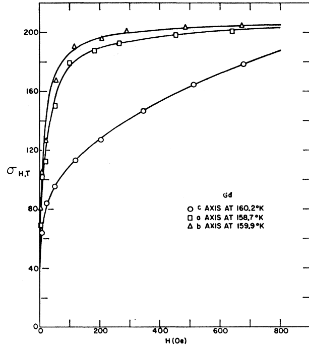
FIG. 2. Magnetic moment per gram versus internal magnetic field for the a -, b -, and c -axis crystals.
