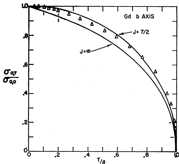
FIG. 6. The reduced spontaneous magnetization curve for the b -axis crystal. The solid lines are for J = 7/2 and J = \infty , from the Weiss quantum theory of ferromagnetism.
