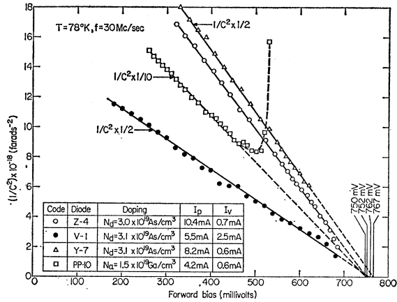
FIG. 3. 1/C^2 versus forward bias voltage for several germanium tunnel diodes. Capacitance built-in voltages are indicated. The large anomalous "inductive" behavior of the p -base unit at high forward bias cannot be accounted for by the package and circuit inductance.
