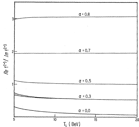
FIG. 1. The ratio \operatorname{Re} f^{(-)} / \operatorname{Im} f^{(-)} as calculated from the forward dispersion relations, for the various sets of \alpha_\rho(0) and \beta_\rho(0) given by von Dardel et al. 4
