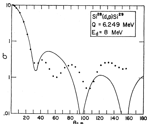
FIG. 10. Angular distributions for the Si^{28}(d,p)Si^{29} , L_N=0 reaction showing the inferior agreement obtained for E_d=8 MeV when a value of V_d is used which is 20 MeV smaller than the value yielding the fit shown in Fig. 7. The parameters are listed in Table IV.
