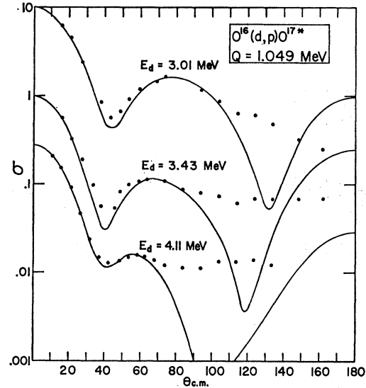
FIG. 2. Comparison of experimental and theoretical angular distributions for the O^{16}(d,p)O^{17*} , L_N=0 reaction for E_d=3.01 , 3.43, and 4.11 MeV. The parameters are listed in Table II.
