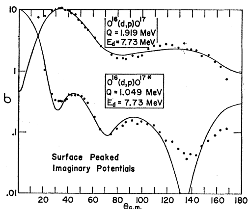
FIG. 23. Results obtained using surface-peaked form factors for W_p and W_d for (top) the \text{O}^{16}(d,p)\text{O}^{17} , L_N = 2 reaction at E_d = 7.73 MeV, and (bottom) the \text{O}^{16}(d,p)\text{O}^{17*} , L_N = 0 reaction at E_d = 7.73 MeV. The parameters are listed in Table V.
