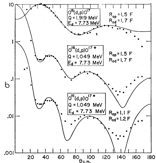
FIG. 22. Angular distributions (top) for the \text{O}^{16}(d,p)\text{O}^{17} , L_N=2 reaction at E_d=7.73 MeV, using large values of R_{0p} and R_{0d} , (middle) for the \text{O}^{16}(d,p)\text{O}^{17*} , L_N=0 reaction at E_d=7.73 MeV, and (bottom) for the \text{O}^{16}(d,p)\text{O}^{17*} , L_N=0 reaction at E_d=7.73 MeV, using small values of R_{0p} and R_{0d} . The parameters are listed in Table V.
