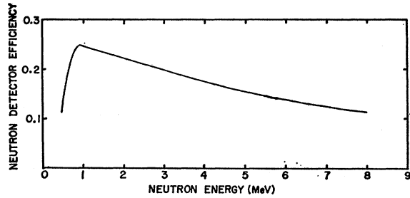
FIG. 5. Measured neutron detection efficiency of the prompt radiation detector.
