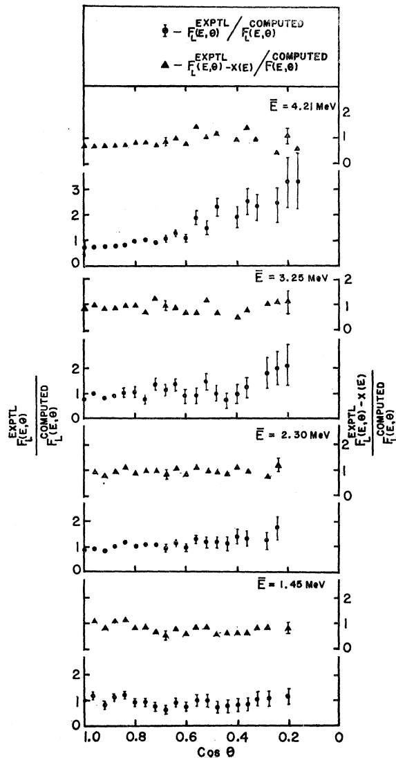
FIG. 13. A plot of F_L^{\text{EXPTL}}(E, \theta)/F_L^{\text{COMPUTED}}(E, \theta) against \cos\theta , showing the deviations of the experimental angular correlations from the computed ones. A plot of [F_L^{\text{EXPTL}}(E, \theta) - X(E)]/F_L^{\text{COMPUTED}}(E, \theta) against \cos\theta also shown in the figure shows that the deviations can be removed after making allowance for the number X(E) of the neutrons emitted prior to scission.
