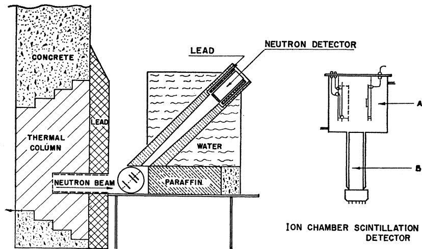
FIG. 1. Diagram of the experimental arrangement.
