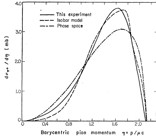
FIG. 10. Pion momentum spectra in the barycentric system
