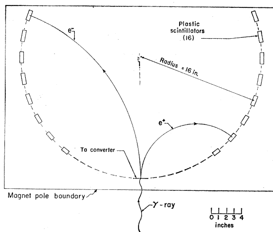
FIG. 3. The circular spectrometer.
