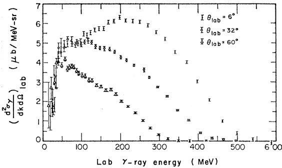
FIG. 6. Gamma-ray energy spectra as measured in the laboratory.
