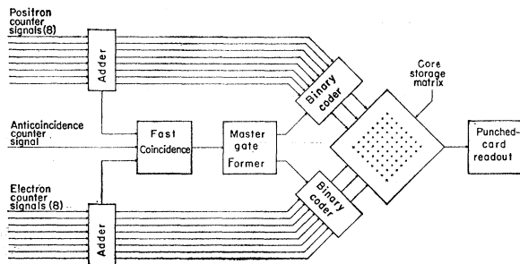
FIG. 4. Block diagram of the electronics.
