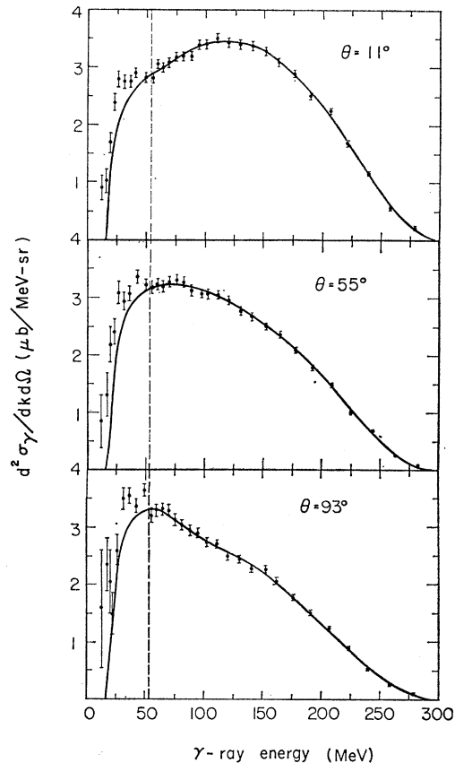
FIG. 7. The gamma-ray spectra after transformation into the barycentric system. All quantities in this figure have been transformed into the barycentric system. The curves represent the gamma-ray spectra resulting from the neutral-pion spectrum giving the best fit to the data as determined by the least-squares analysis. Data to the left of the vertical dashed line were not included in this analysis.
