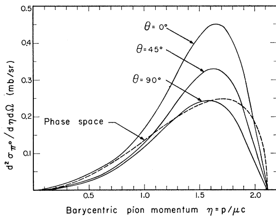
FIG. 8. The neutral-pion spectra in the barycentric system which give the gamma-ray spectra plotted in Fig. 6. The dashed curve represents the pion spectrum given by the three-body final-state phase space. It is normalized to give the same total cross section as the solid curves, assuming an isotropic angular distribution.
