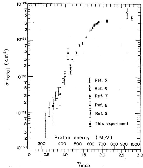
FIG. 1. Total cross section for the reaction p+p \rightarrow p+p+\pi^0 . \eta_{\max} is the maximum pion momentum in the barycentric system, in units of m_{\pi^0}c .
