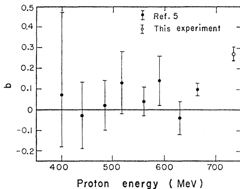
FIG. 9. Values of the coefficient b in the expansion d\sigma_{\pi^0}/d\Omega \propto \frac{1}{2} + b \cos^2\theta .
