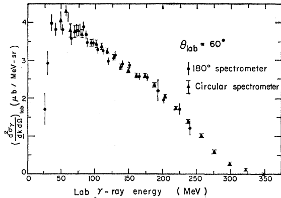
FIG. 5. Spectra obtained with the circular spectrometer and the 180-deg spectrometer, plotted separately.
