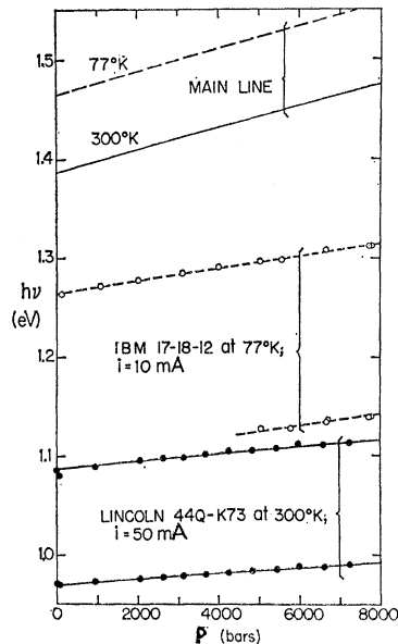
FIG. 6. Variation with pressure of the peak energy of subsidiary lines from the IBM and Lincoln diodes.
