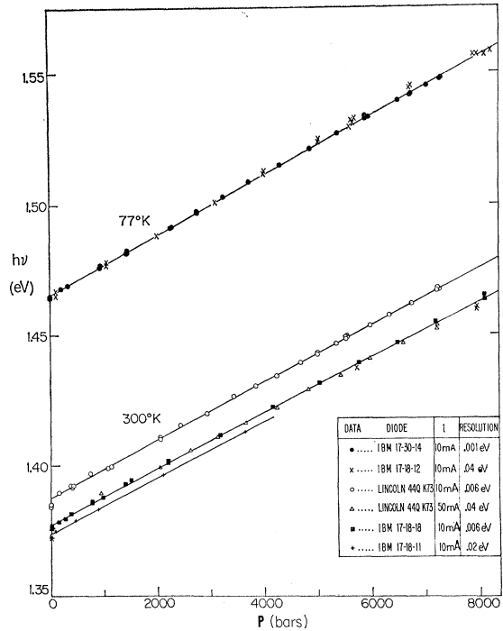
FIG. 5. Variation with pressure of the peak energy of the spontaneous emission line.
