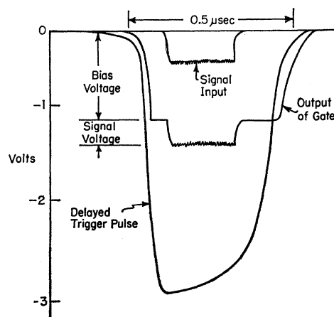
FIG. 3. Illustration of width and amplitudes of gate and signal pulses.
