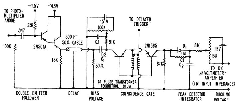
FIG. 2. Circuit diagram of special components of pulse-detection system.
