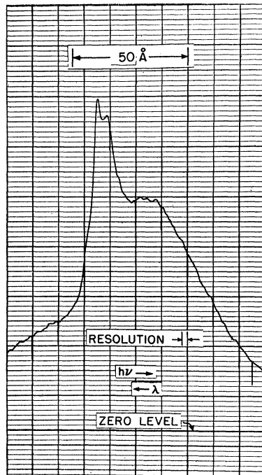
FIG. 4. Typical recording of spectrum of stimulated emission.
