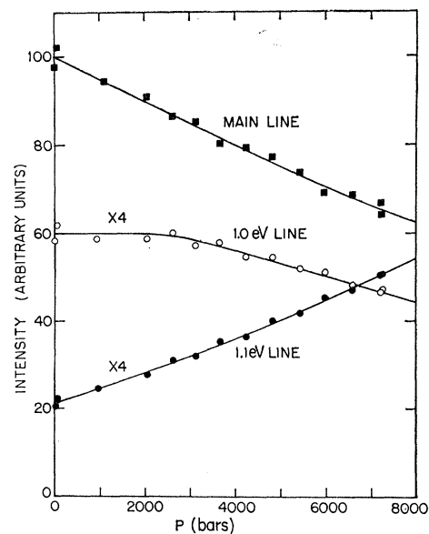
FIG. 7. Variation with pressure of the relative peak intensities of the main and two subsidiary lines from the Lincoln diode at 300°K.
