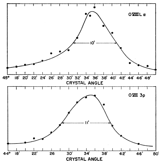
FIG. 6. Observed line profiles of O VIII L_\alpha and O VII 1s^2 1s_0-1s_3p^2 1P_1 . The reduction of the observed width to a Doppler temperature is explained in the text.
