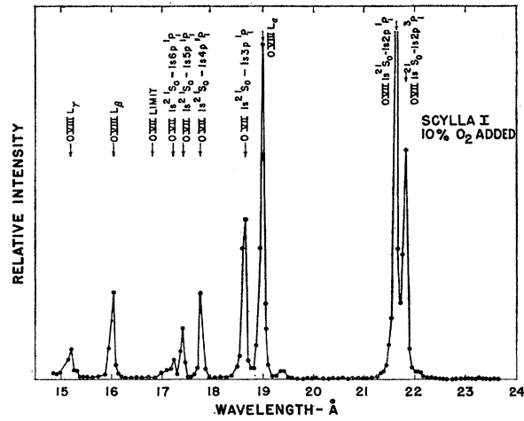
FIG. 3. Line spectrum observed with the KAP crystal. The arrows indicating the identified lines of wall impurities are at the predicted wavelengths of the lines.
