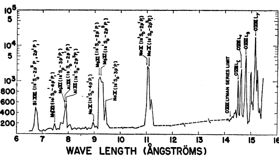
FIG. 2. Line spectrum observed with the beryl crystal. The arrows indicating the identified lines of wall impurities are at the predicted wavelengths of the lines. Intensity scale is relative.
