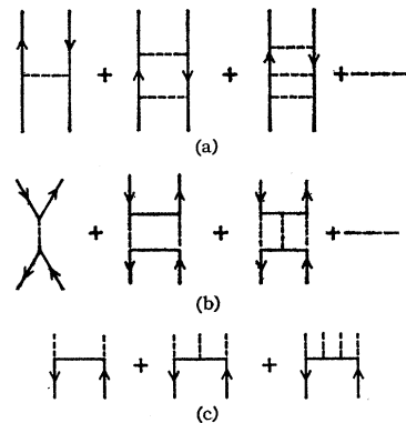
FIG. 1. (a) The ladder diagrams in the s channel. (b) The annihilation-recreation scattering diagrams in the crossed channel. (c) N\bar{N} annihilation into mesons.
