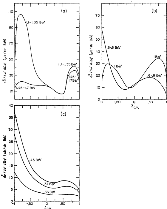
FIG. 3. Calculated angular distributions of the inelastically scattered projectile pion in the center-of-mass system for the processes \pi^- p \rightarrow \pi^- p \pi_{\text{soft}}^0 and \pi^+ p \rightarrow \pi^+ n \pi_{\text{soft}}^- when the soft pion is emitted in accompaniment with the outgoing nucleon. The curves are labeled by the incident kinetic energies in the laboratory system. When the soft pion emitted is charged, the ordinate scale should be multiplied by 2. These calculations are based directly on elastic \pi^- p scattering data as given in Ref. 17.
