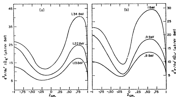
FIG. 5. Calculated angular distributions of the inelastically scattered projectile pion in the center-of-mass system for the processes \pi^+p \rightarrow \pi^+p\pi_{soft}^0 and \pi^-p \rightarrow \pi^-p\pi_{soft}^+ . (a) shows the distributions for when the soft pion is emitted in accompaniment of the outgoing nucleon, and (b) shows the distribution for emission of soft pions in the laboratory frame. The number labeling each curve refers to the incident kinetic energy in the laboratory. For emission of charged soft pions the ordinate scales must be read larger by a factor of 2. These calculations are based directly on elastic \pi^+p scattering data as given in Ref. 17.
