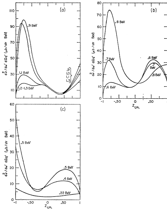
FIG. 4. Angular distributions for the same processes as are described for Fig. 3 except that here the emitted pions are "soft" in the laboratory frame instead of in the rest frame of outgoing nucleon.
