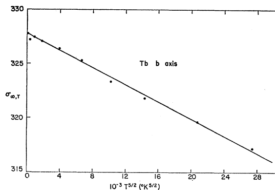
FIG. 9. Saturation magnetization of the b -axis crystal vs T^{5/2} .
