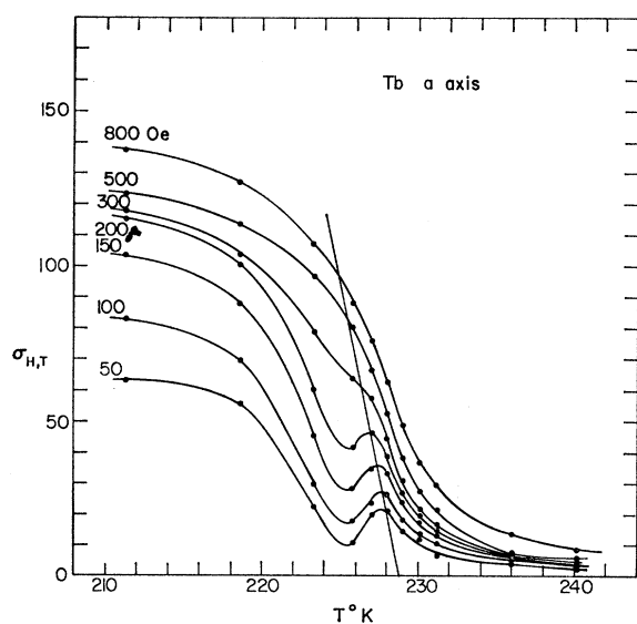
FIG. 3. Magnetic moment/g vs temperature for the a -axis crystal in the neighborhood of the Néel point. External fields are indicated.
