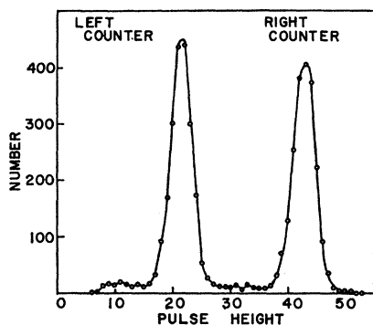
FIG. 2. Pulse-height distribution of protons scattered into the left and right counter telescopes from copper at \theta(\text{c.m.}) = 45^\circ .
