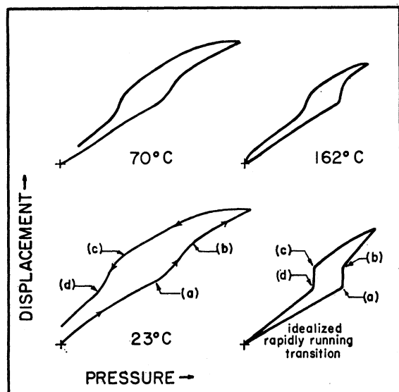
FIG. 1. Displacement vs pressure for HgTe at 23, 70, and 162 ^{\circ}\text{C} . For comparison with these sluggish transitions, the idealized course of a rapidly running transition is also portrayed.
