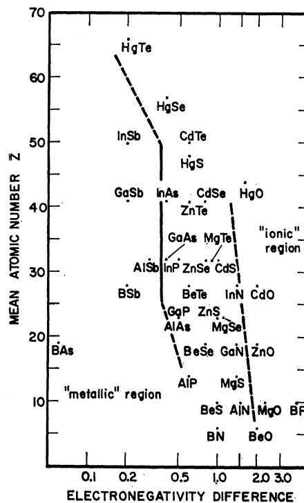
FIG. 5. Electronegativity difference, after Haissinsky (reference 20), plotted vs mean atomic number, \bar{Z} , for III-V and II-VI compounds. The classification into "metallic" intermediate and "ionic" regions is discussed in the text.
