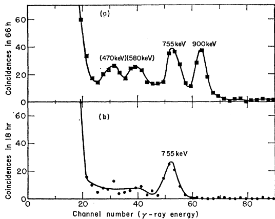
FIG. 12. Gamma-ray spectrum of \text{Cm}^{242} , containing a few percent \text{Cm}^{248} , in coincidence with alpha particles (see Fig. 10): (a) in coincidence with 5.18-MeV alpha particles, (b) in coincidence with 5.27-MeV alpha particles.
