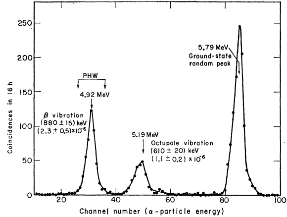
FIG. 7. Alpha spectrum of \text{Cm}^{244} in coincidence with gamma rays > 480 keV. PHW refers to the pulse-height window used when recording the gamma rays in coincidence with the 4.92-MeV alpha groups (see Fig. 8).
