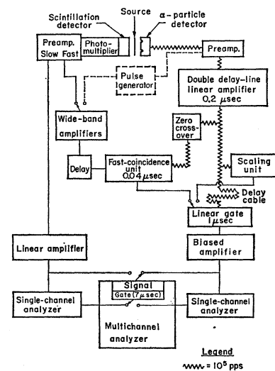
FIG. 2. Simplified block diagram of the electronic apparatus used in the experiments with silicon semiconductor alpha detectors.
