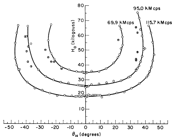
FIG. 11. Angular dependence of AFMR at 77°K. The points with horizontal and vertical bars correspond to additional low-intensity resonances observed at 69.9 kMc/sec and 95.0 kMc/sec, respectively.
