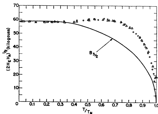
FIG. 9. Calculated values of (2\lambda K)^{1/2} vs temperature derived from Figs. 7 and 8. The triangles and circles correspond to 70.7 and 36.0 kMc/sec, respectively, and the solid line is the associated Brillouin function for S=3/2 .
