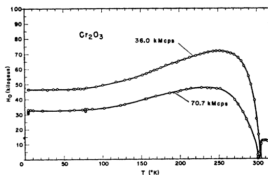
FIG. 7. Temperature dependence of AFMR in Cr 2 O 3 at 36.0 and 70.7 kMc/sec for H_0 parallel to the c axis.
