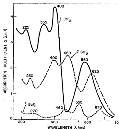
Fig. 2. Absorption of irradiated ( 5\times 10^6 rad): (1) Harshaw \text{CaF}_2 ( 5\times 10^{-4}\% Y); (2) single crystal \text{SrF}_2 (0.2% Y); (3) single crystal \text{BaF}_2 (0.2% Y). These materials color as follows: \text{CaF}_2(\text{Y}) —blue; \text{SrF}_2(\text{Y}) —green; and \text{BaF}_2(\text{Y}) —red.
