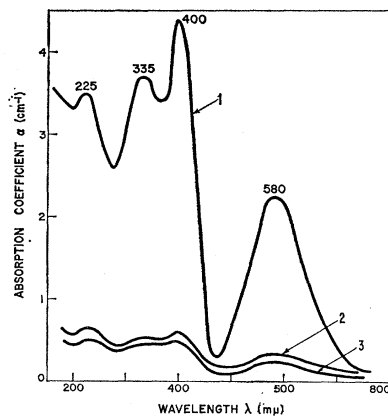
FIG. 1. Absorption of irradiated ( 5 \times 10^6 rad) materials: (1) Harshaw \text{CaF}_2 ( 5 \times 10^{-4}\% Y); (2) a crystal grown from Baker, reagent grade \text{CaF}_2 ; (3) a crystal grown from \text{CaF}_2 , synthesized from pure \text{CaCO}_3 by Dr. A. Wold, Lincoln Laboratory. The Y contamination of crystals (2) and (3) is less than 1 part per million.
