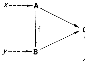
FIG. 1. Generalized decay chain used in defining terms of Eq. (1).
