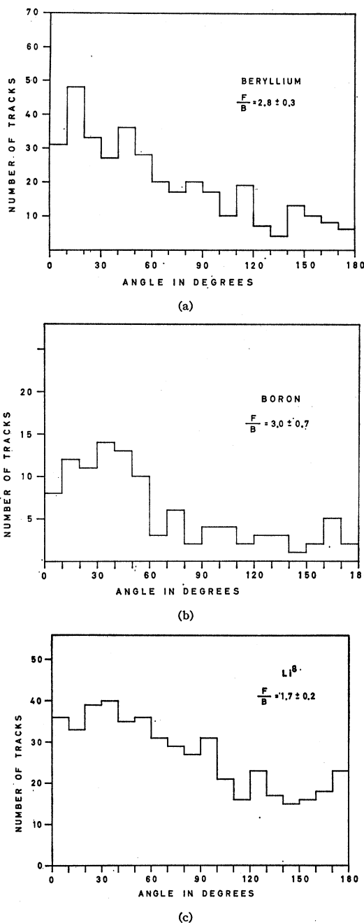
FIG. 7. Angular distribution of (a) Be fragments of range R > 40 \mu ; (b) B fragments of range R > 40 \mu ; (c) \text{Li}^8 fragments. F/B give the forward/backward ratio.
