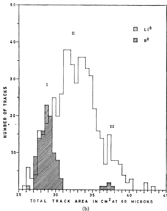
FIG. 3. Histogram showing the projected total track area of the last 60 \mu of hammer tracks, corrected for depth in the emulsions and illumination conditions.
