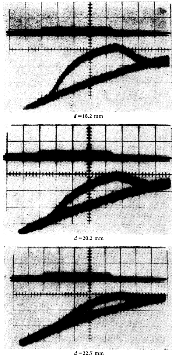
FIG. 4. Photographs of oscilloscope traces showing a typical sequence of quenched light signals at various distances d from the heated region for a cylindrical plasma. The discharge parameters are: Neon gas at 7 mm Hg, 200 \mu\text{sec} in the afterglow, H = 660 Oe, n = 5.5 \times 10^{11}/\text{cm}^3 . The time scale is 5 \mu\text{sec}/\text{cm} .
