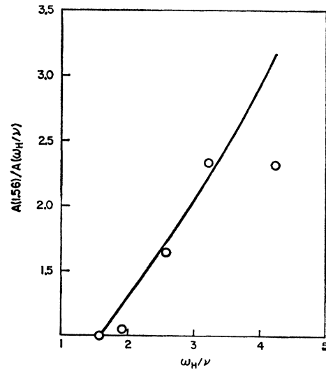
FIG. 8. The ratio A(1.56)/A(\omega_H/\nu) (neglecting the temperature dependence of \kappa_{xx}/\kappa_0 ) for the cylindrical plasma as a function of \omega_H/\nu . The experimental points (O) refer to neon afterglow plasma at 7.7 mm of Hg with H=1125 Oe. The solid line is the theoretical curve.
