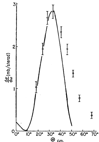
FIG. 23. Angular distribution of tritons from O 18 (p,t)O 16 ground state. The solid line is Cj_0^2(qr_0) curve with C chosen to give fit on small-angle data; l=0 , r_0=6.2 F. Proton energy was 17.6 MeV.
