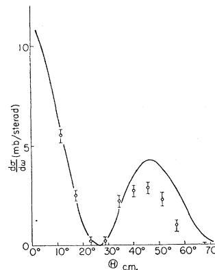
FIG. 15. Angular distribution of tritons from C 14 (p, t)C 12 ground state. The solid line is a Cj_0^2(qr_0) curve with C chosen to give fit on side of first maximum; l=0 , r_0=5.1 F. Proton energy was 18.5 MeV.
