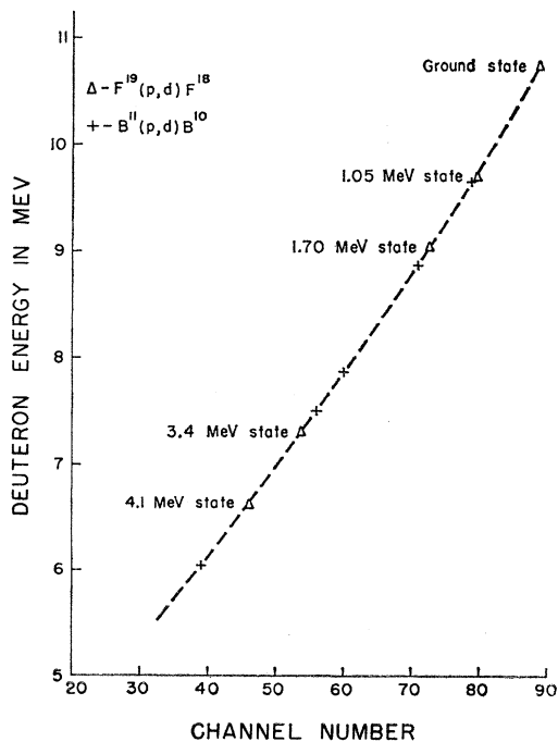
FIG. 4. Energy calibration for B^{11}(p,d)B^{10} . This is an example of the calibration curves used in these experiments. The F^{19}(p,d)F^{18} reaction was used as an energy standard.
