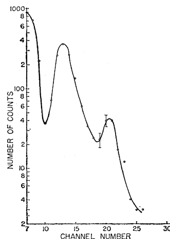
FIG. 2. Multiplied pulse spectrum for O^{18} at 20^\circ lab. This is a spectrum displayed on 20-channel analyzer as it was used to select deuterons and tritons. Part of the proton peak falls below the lower level of the 20 channels analyzed.
