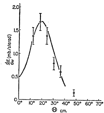
FIG. 8. Angular distribution of deuterons from B 11 (p,d)B 10* 2.15-MeV state. The solid line is a plane-wave Butler curve with l=1 , r_0=6.0 F. Proton energy was 19.0 MeV.
