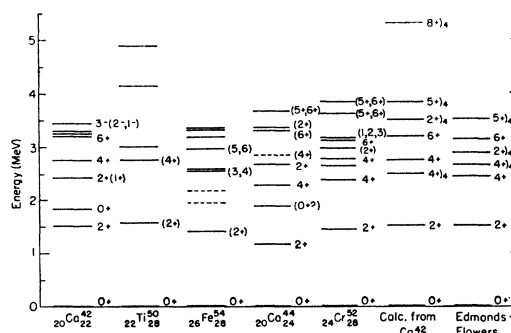
Fig. 5. Experimental and predicted level structures of even- A , single-closed-shell nuclides in the f_{7/2} region. Ca^{42} , this work; Ti^{50} and Fe^{54} , reference 28; Ca^{44} , reference 29; Cr^{52} , reference 30.
