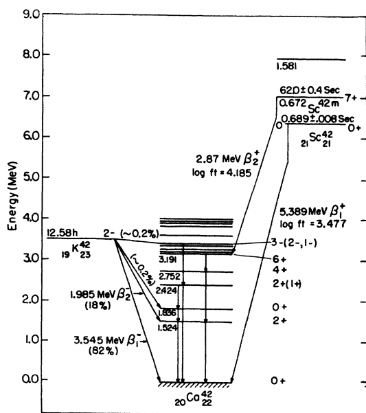
Fig. 4. Level structure of Ca^{42} and proposed decay scheme of Sc^{42m} with data from the K^{42} decay (references 10, 11).
