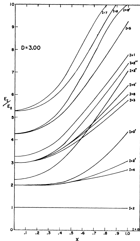
FIG. 4. Here D = 3.00 and 0 \leq x \leq 1.0 .
