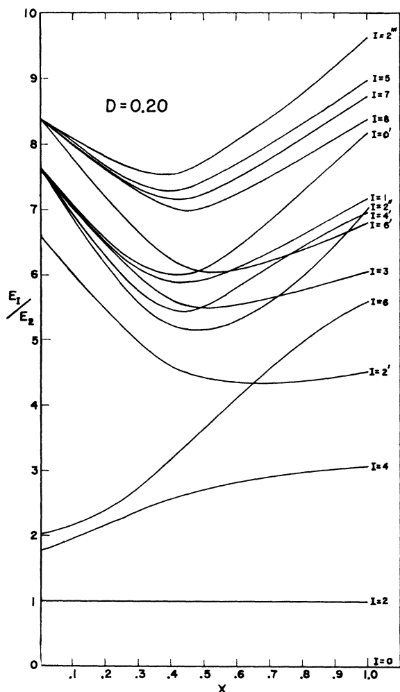
FIG. 1. The computed variation of the ratio of the energy of the level of spin I ( E_I ) to the energy of the first excited state ( E_2 ). The calculation is for D=0.20 and 0 \leq x \leq 1.0 . [The shell-model states are (\frac{1}{2})_{0,2,4,6} with surface interaction included.]
