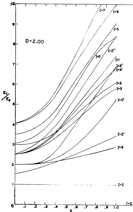
FIG. 3. Here D = 2.00 and 0 \leq x \leq 1.0 .
